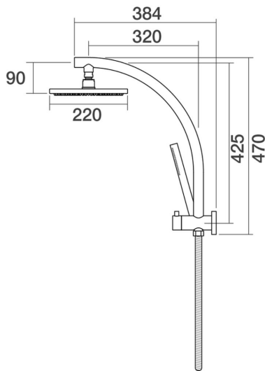
Lugano Wall Shower Divertor High Rise Arc C22.061.3.01 - Chrome
