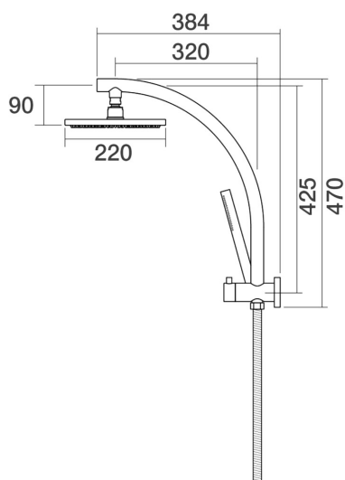
Lugano Wall Shower Divertor High Rise Arc C22.061.3.43 - Brass
