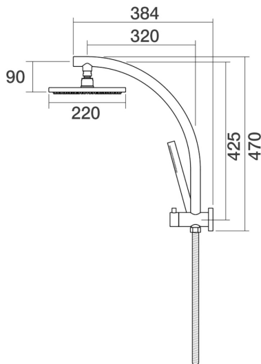
Lugano Wall Shower Divertor High Rise Arc C22.061.3.75 - Forest Mist
