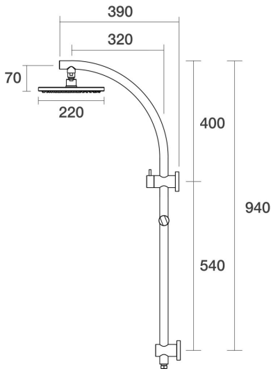
Lugano Wall Shower Divertor on Rail Arc Top Connection C22.063.1.01 - Chrome
