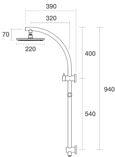
Lugano Wall Shower Divertor on Rail Arc Top Connection C22.063.1.02 - Brushed Chrome
