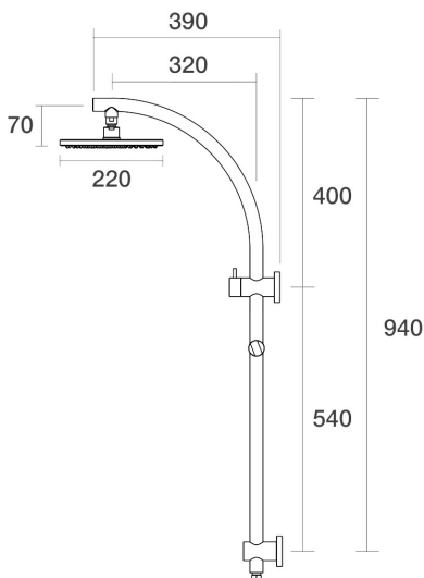
Lugano Wall Shower Divertor on Rail Arc Top Connection C22.063.1.42 - Brushed Copper
