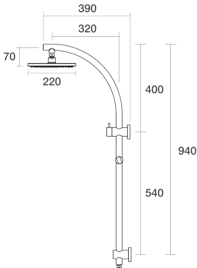
Lugano Wall Shower Diverter on Rail Arc Top Connection C22.063.1.43 - Brass
