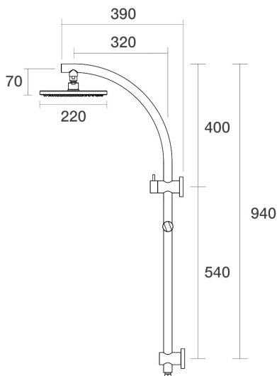
Lugano Wall Shower Divertor on Rail Arc Top Connection C22.063.1.48 - Copper
