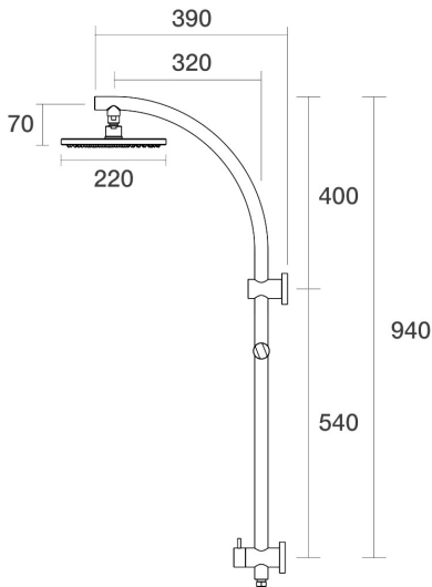
Lugano Wall Shower Divertor on Rail Arc Bottom Connection C22.063.2.42 - Brushed Copper
