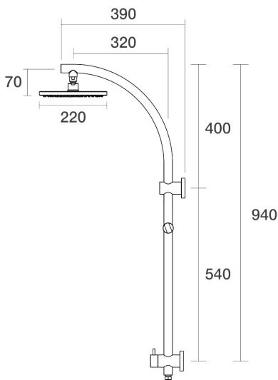
Lugano Wall Shower Diverter on Rail Arc Bottom Connection C22.063.2.43 - Brass
