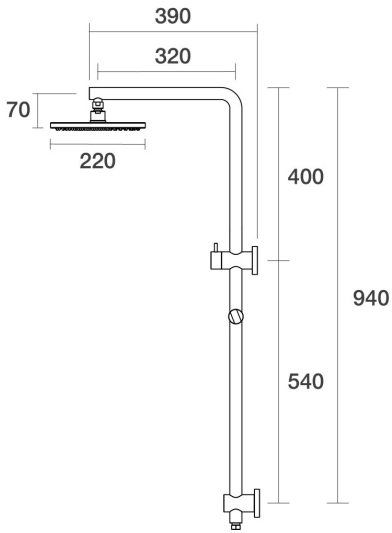
Lugano Wall Shower Divertor on Rail 90 Degree Top Connection
