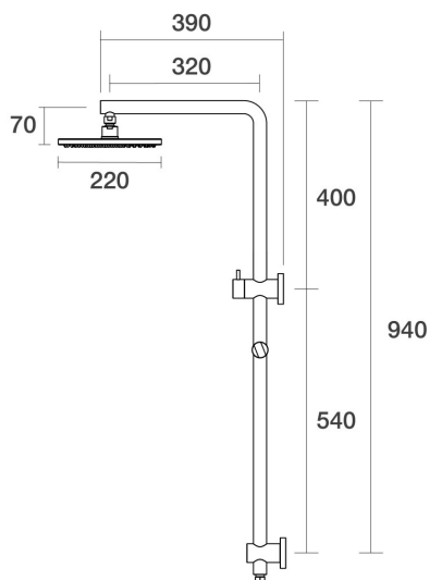
Lugano Wall Shower Diverter on Rail 90 Degree Top Connection C22.063.3.34 - Matt Black
