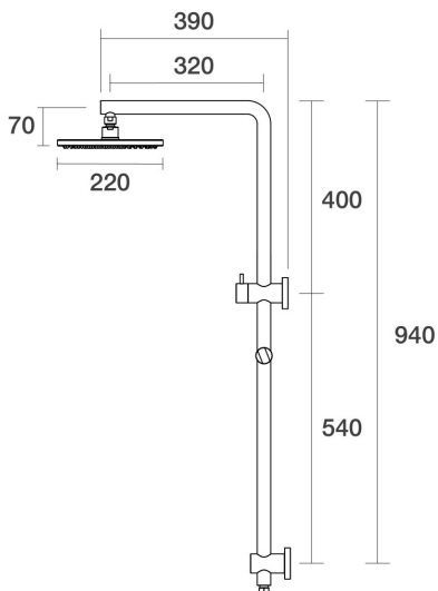
Lugano Wall Shower Diverter on Rail 90 Degree Top Connection C22.063.3.41 - Brushed Brass
