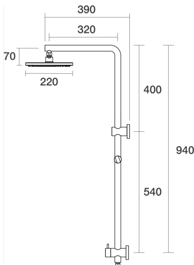
Lugano Wall Shower Divertor on Rail 90 Degree Bottom Connection C22.063.4.01 - Chrome
