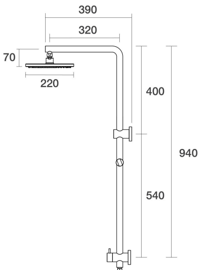
Lugano Wall Shower Divertor on Rail 90 Degree Bottom Connection C22.063.4.23 - Gunmetal
