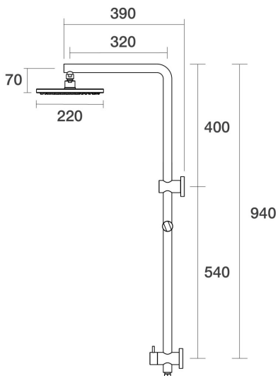
Lugano Wall Shower Divertor on Rail 90 Degree Bottom Connection C22.063.4.48 - Copper
