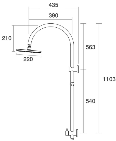
Lugano Wall Shower Divertor on Rail Gooseneck Bottom Connection C22.063.6.01 - Chrome
