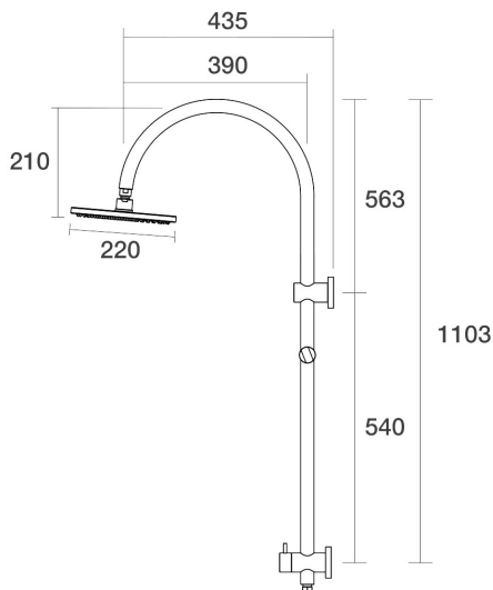
Lugano Wall Shower Diverter on Rail Gooseneck Bottom Connection C22.063.6.34 - Matt Black
