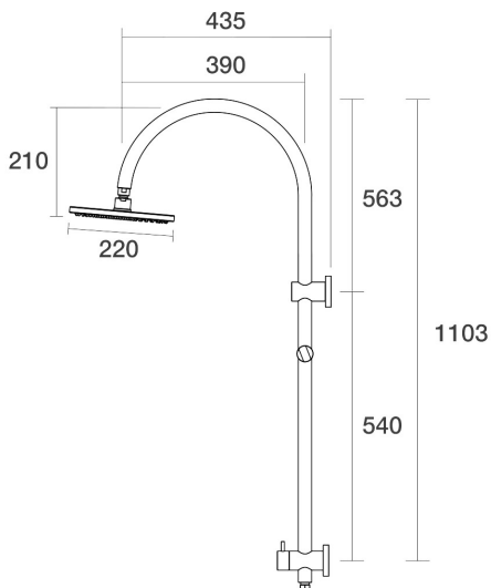
Lugano Wall Shower Diverter on Rail Gooseneck Bottom Connection C22.063.6.42 - Brushed Copper
