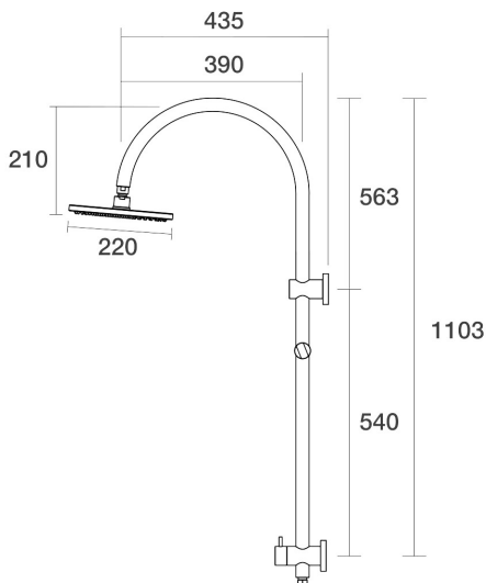
Lugano Wall Shower Divertor on Rail Gooseneck Bottom Connection C22.063.6.48 - Copper
