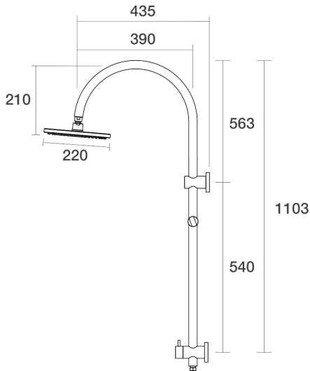
Lugano Wall Shower Divertor on Rail Gooseneck Bottom Connection C22.063.6.52 - Burnished
