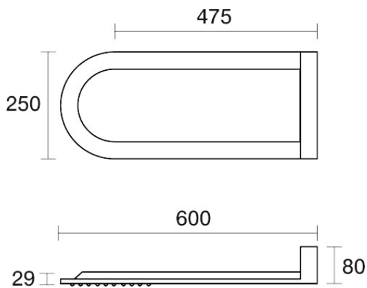
Lava Fixed Wall Arm Shower 475mm C23.011.1.19 - 23k Brushed Brass Gold
