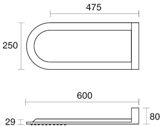
Lava Fixed Wall Arm Shower 475mm C23.011.1.45 - Native Brass
