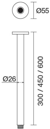
Fuze Ceiling Fixed Dropper 300mm C25.041.2.01 - Chrome
