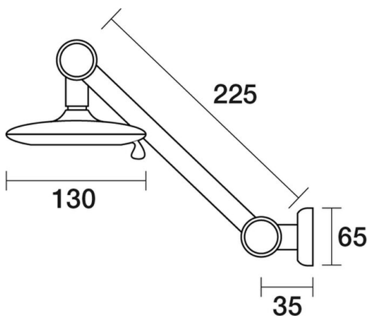
Portsea Wall Adjustable Arm Five Function Rose 260mm reach C29.071.1.01 - Chrome
