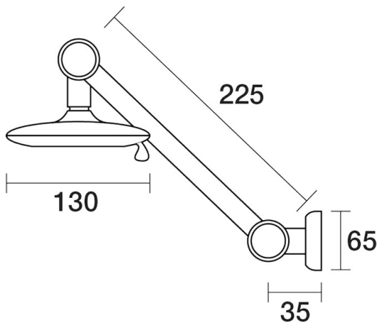
Portsea Wall Adjustable Arm Five Function Rose 260mm reach
