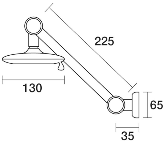
Portsea Wall Adjustable Arm Five Function Rose 260mm reach C29.071.1.34 - Matt Black
