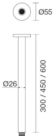
Tudor Ceiling Dropper 300mm C31.041.2.04 - Chrome / Ivory
