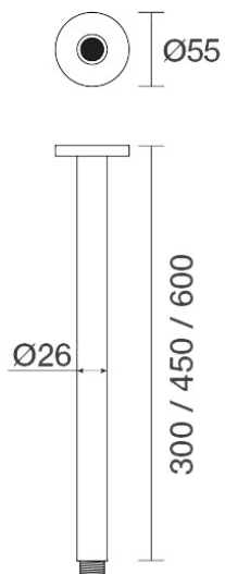
Tudor Ceiling Dropper 450mm C31.041.3.47 - Luminick
