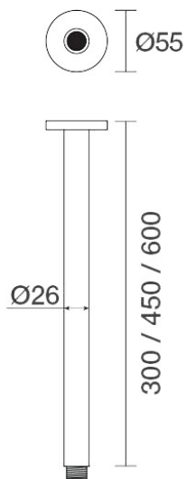
Tudor Ceiling Dropper 600mm C31.041.4.23 - Gunmetal
