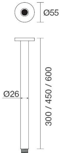
Tudor Ceiling Dropper 600mm C31.041.4.40 - Rumbled Brass
