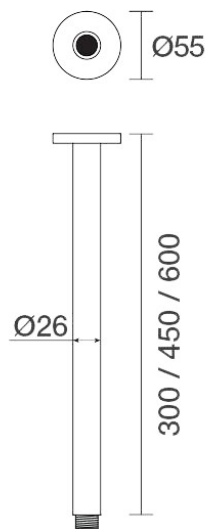
Tudor Ceiling Dropper 600mm C31.041.4.54 - Volcanic Grey
