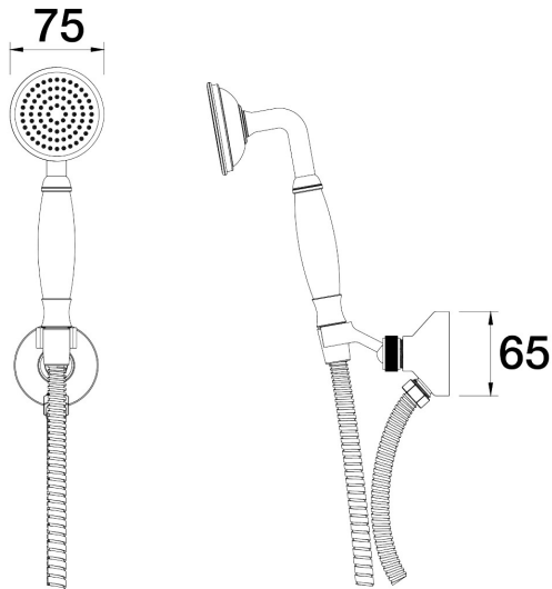
Tudor Handshower on Wall Bracket Single Function Porcelain Handle C31.051.1.11 - 23k Gold
