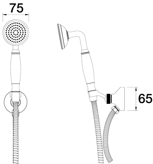
Tudor Handshower on Wall Bracket Single Function Porcelain Handle C31.051.1.27 - Satin Pearl
