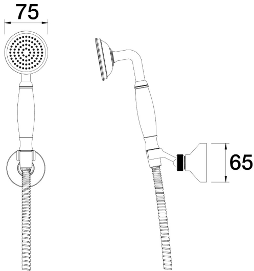
Tudor Handshower on Wall Bracket Without water connection Porcelain Handle C31.051.2.32 - Midnight Black
