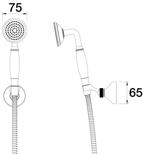
Tudor Handshower on Wall Bracket Without water connection Porcelain Handle C31.051.2.54 - Volcanic Grey
