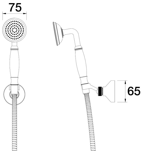
Tudor Handshower on Wall Bracket Without water connection Porcelain Handle C31.051.2.57 - Matt Nickel
