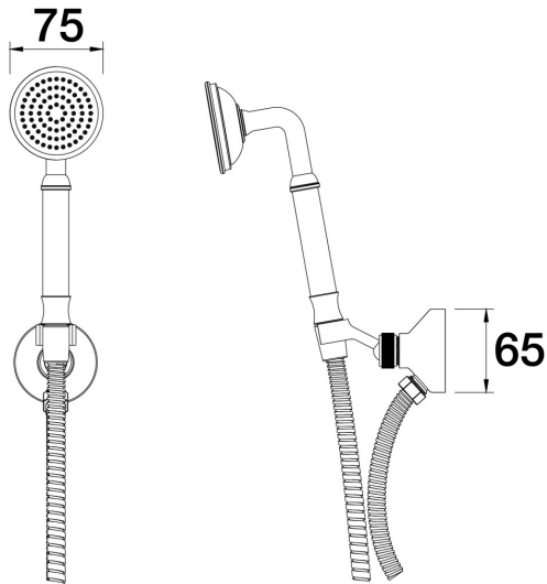
Tudor Handshower on Wall Bracket Single Function with Brass Handle C31.051.3.03 - Chrome / White
