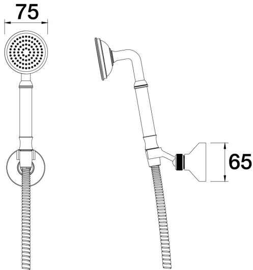
Tudor Handshower on Wall Bracket Without water connection with Brass handle C31.051.4.21 - Brushed Rose Gold
