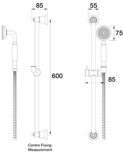
Tudor Handshower on Rail Single Function Porcelain Handle C31.052.1.04 - Chrome / Ivory
