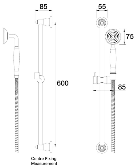
Tudor Handshower on Rail Single Function Porcelain Handle C31.052.1.54 - Volcanic Grey
