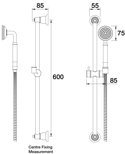
Tudor Handshower on Rail Single Function with Brass Handle C31.052.2.52 - Burnished
