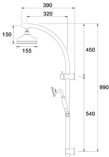
Tudor Wall Shower Diverter on Rail Arc Top Connection Porcelain Handle C31.063.1.03 - Chrome / White
