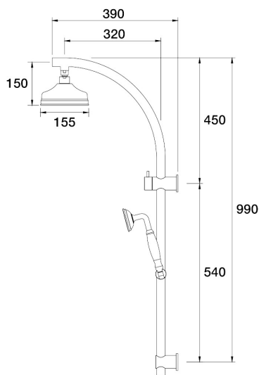
Tudor Wall Shower Diverter on Rail Arc Top Connection Porcelain Handle C31.063.1.26 - Black Sapphire
