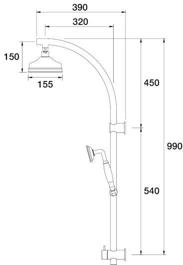
Tudor Wall Shower Divertor on Rail Arc Bottom Connection Porcelain Handle C31.063.2.01 - Chrome
