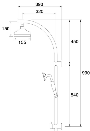
Tudor Wall Shower Divertor on Rail Arc Bottom Connection Porcelain Handle C31.063.2.27 - Satin Pearl
