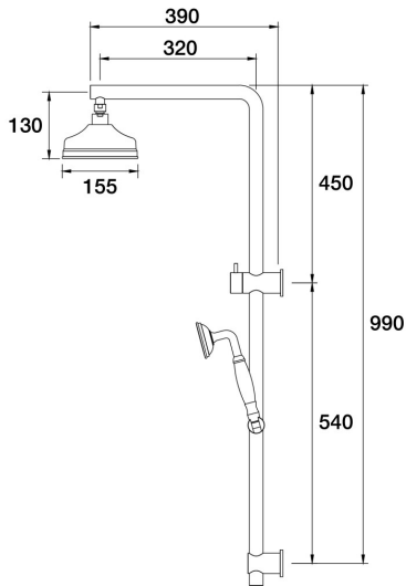
Tudor Wall Shower Diverter on Rail 90 Degree Top Connection Porcelain Handle C31.063.3.15 - Gold / Apricot
