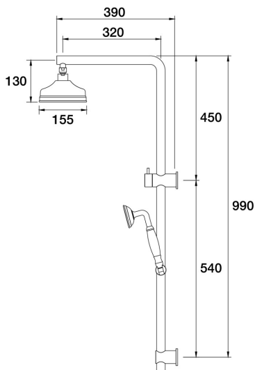
Tudor Wall Shower Divertor on Rail 90 Degree Top Connection Porcelain Handle C31.063.3.54 - Volcanic Grey
