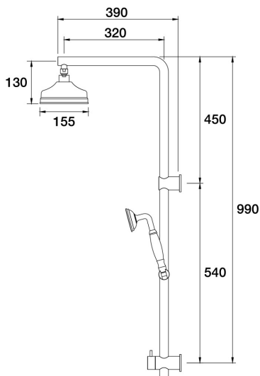
Tudor Wall Shower Divertor on Rail 90 Degree Bottom Connection Porcelain Handle C31.063.4.11 - 23k Gold
