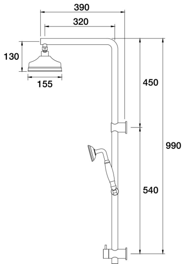
Tudor Wall Shower Diverter on Rail 90 Degree Bottom Connection Porcelain Handle C31.063.4.43 - Brass
